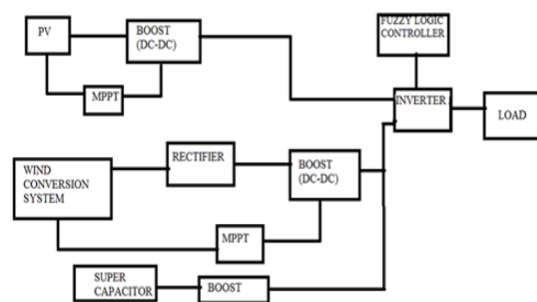
Figure 1. Proposed block diagram.
