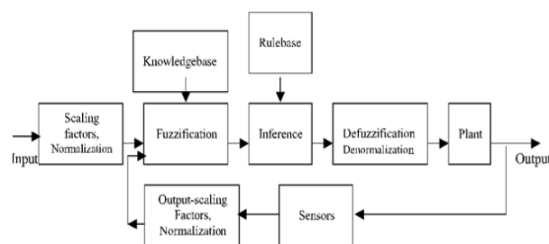
Figure 2. FLC controlling strategy.
