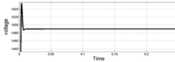
Figure10. Wind dc-dc converter output voltage.
