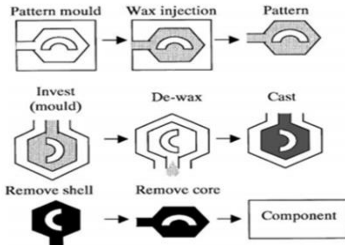
Fig.1 Basic Principle of Investment Casting
